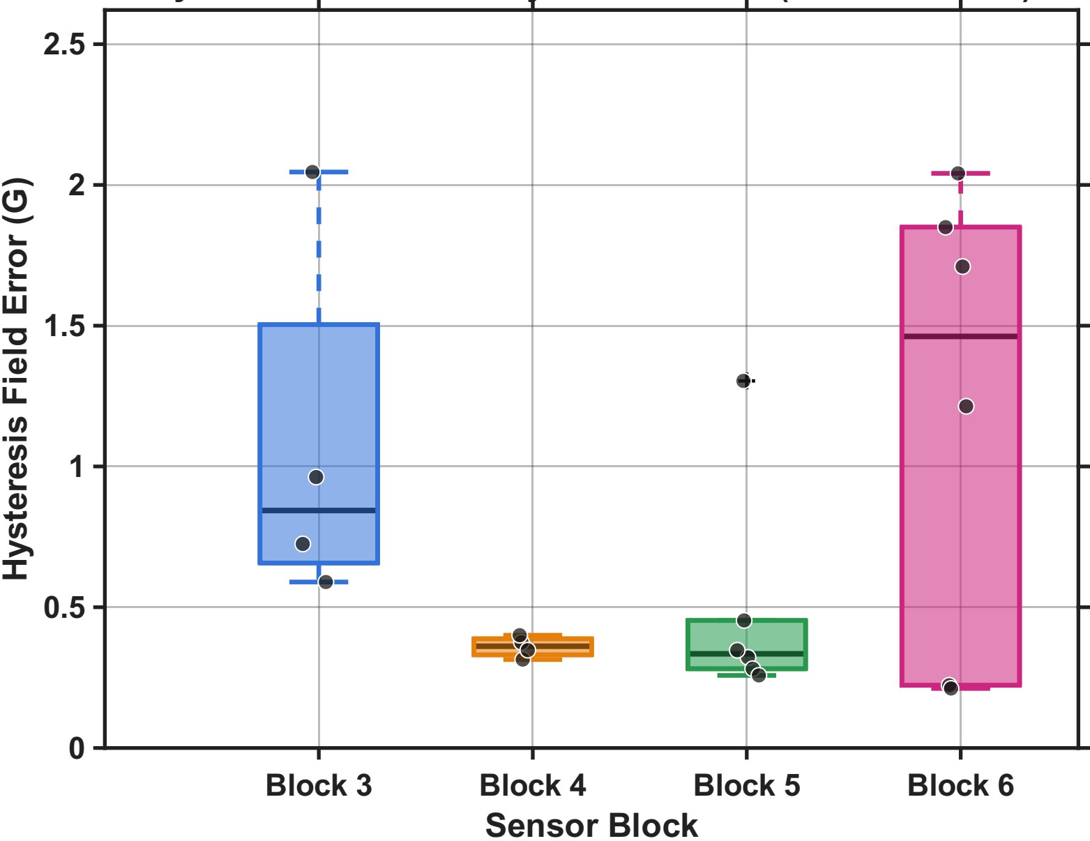
Hysteresis Field Error by Sensor Block (Lower = Better)
